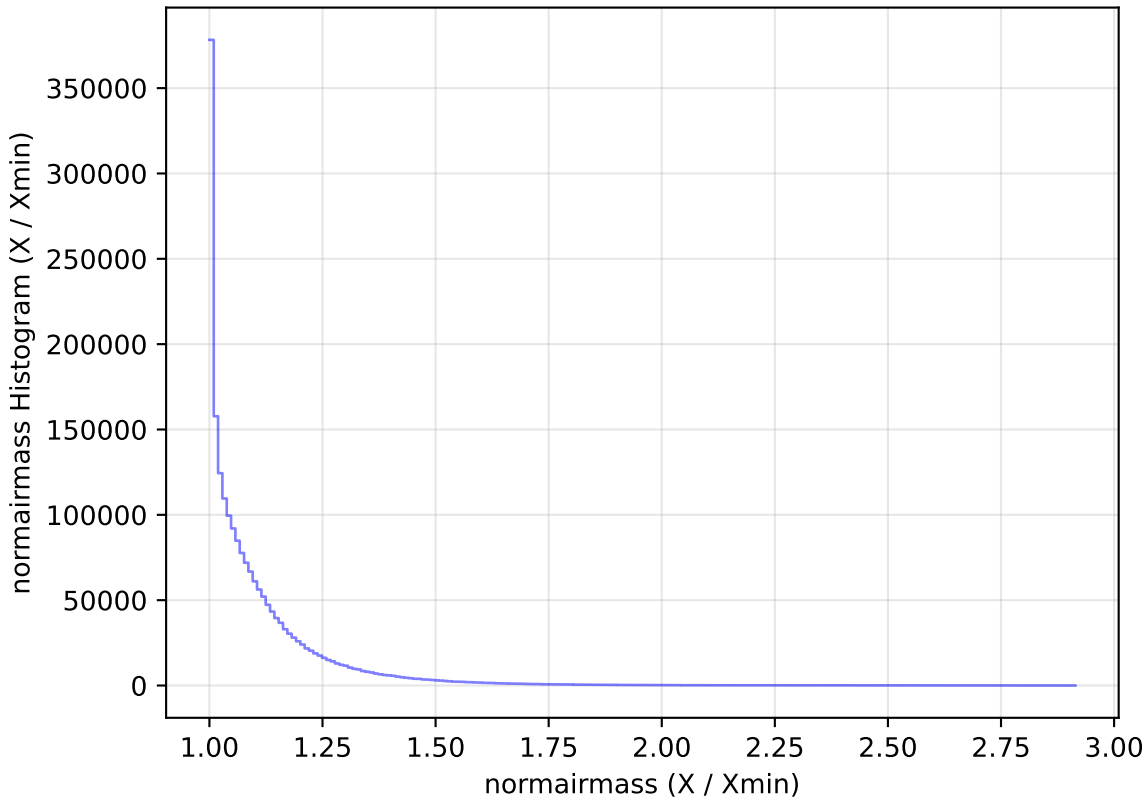
baseline_v2.1_10yrs WFD all bands: normairmass Histogram
