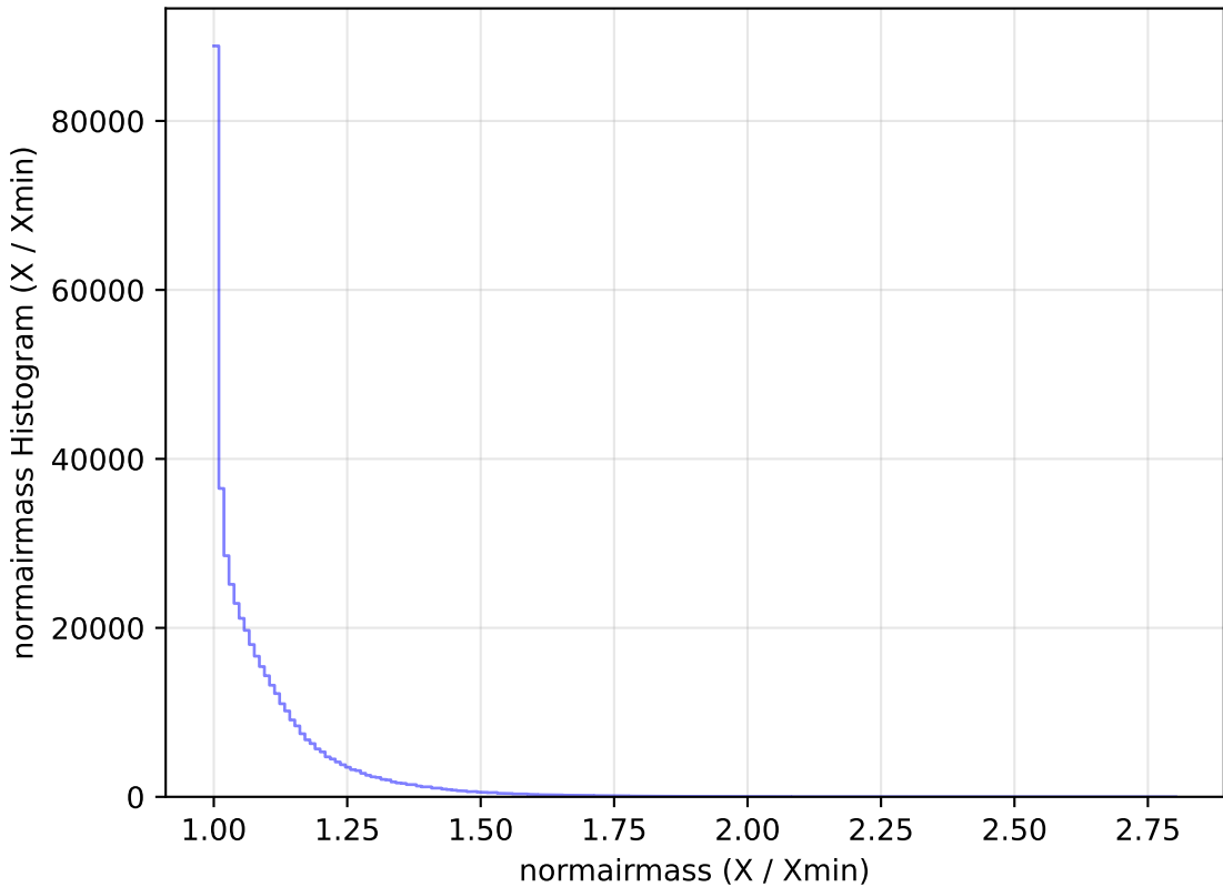
baseline_v2.1_10yrs All sky i band: normairmass Histogram
