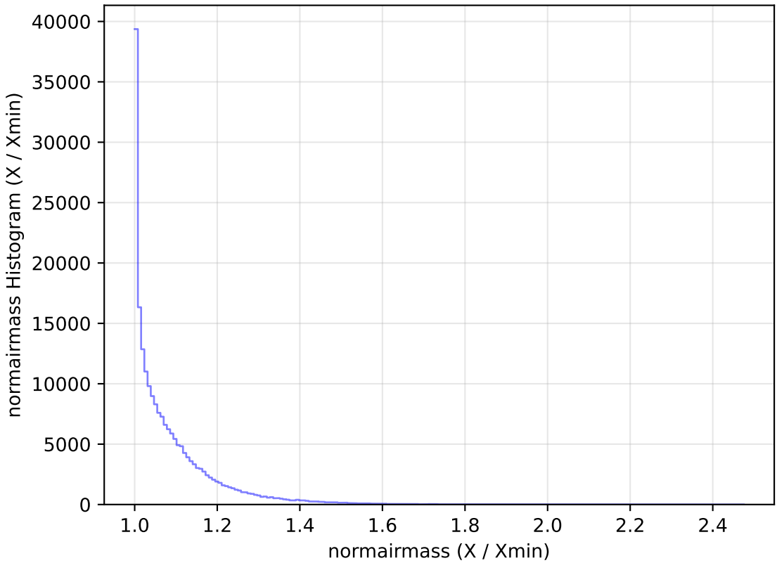
baseline_v2.1_10yrs All sky g band: normairmass Histogram
