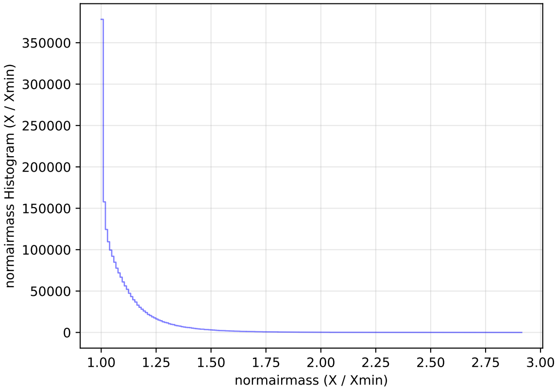
baseline_v2.1_10yrs All sky all bands: normairmass Histogram
