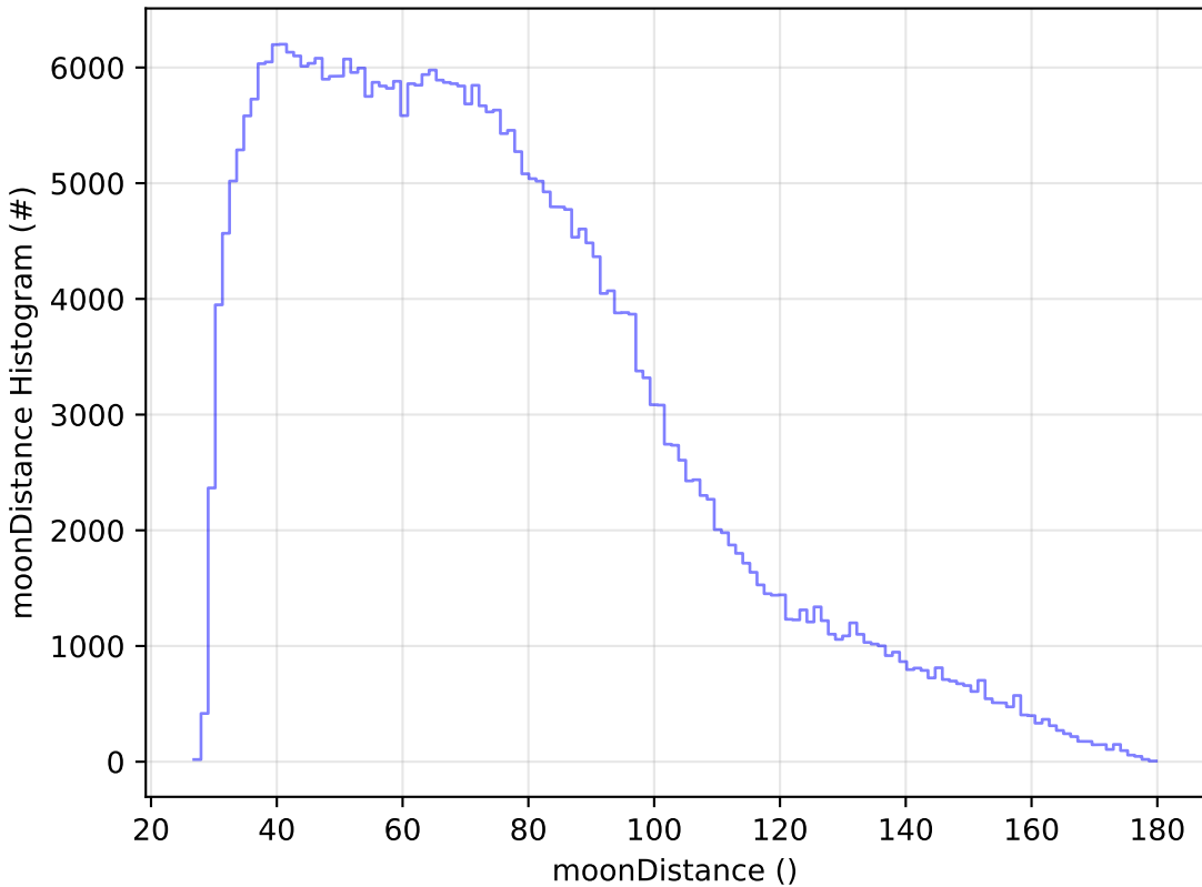
baseline_v2.1_10yrs WFD z band: moonDistance Histogram
