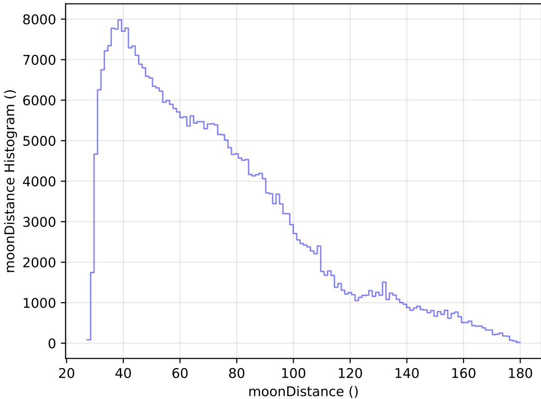
baseline_v2.1_10yrs WFD y band: moonDistance Histogram
