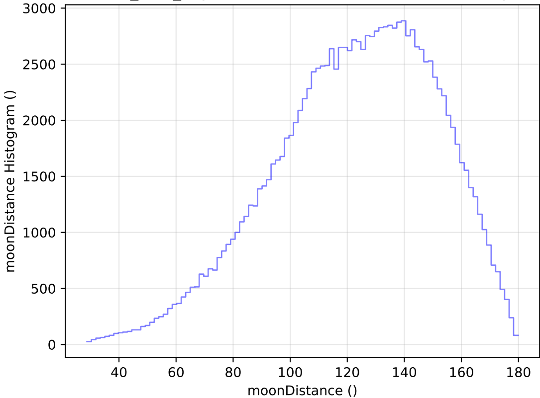
baseline_v2.1_10yrs WFD u band: moonDistance Histogram
