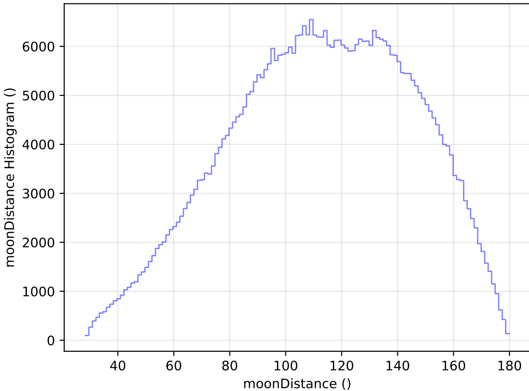
baseline_v2.1_10yrs WFD r band: moonDistance Histogram
