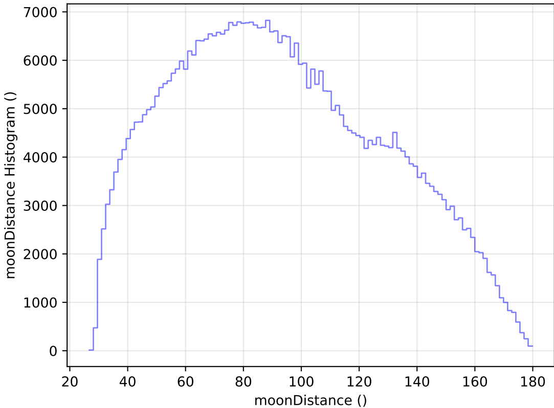
baseline_v2.1_10yrs WFD i band: moonDistance Histogram
