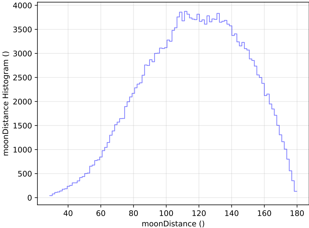
baseline_v2.1_10yrs WFD g band: moonDistance Histogram
