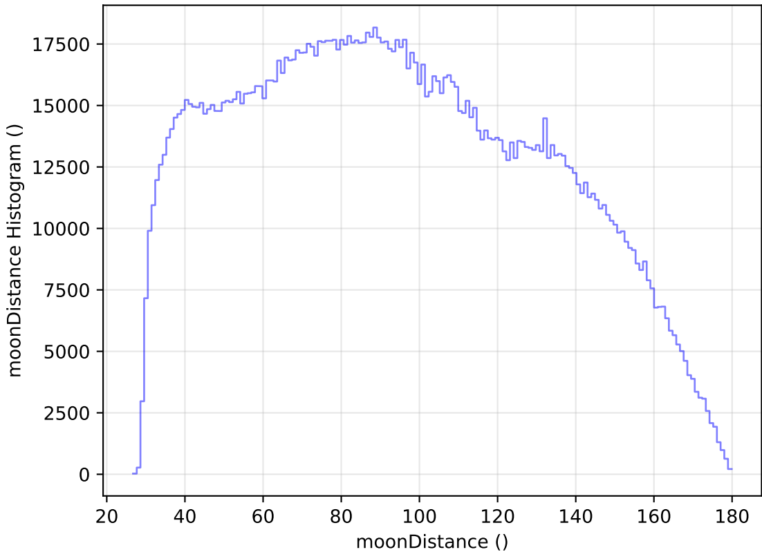
baseline_v2.1_10yrs WFD all bands: moonDistance Histogram
