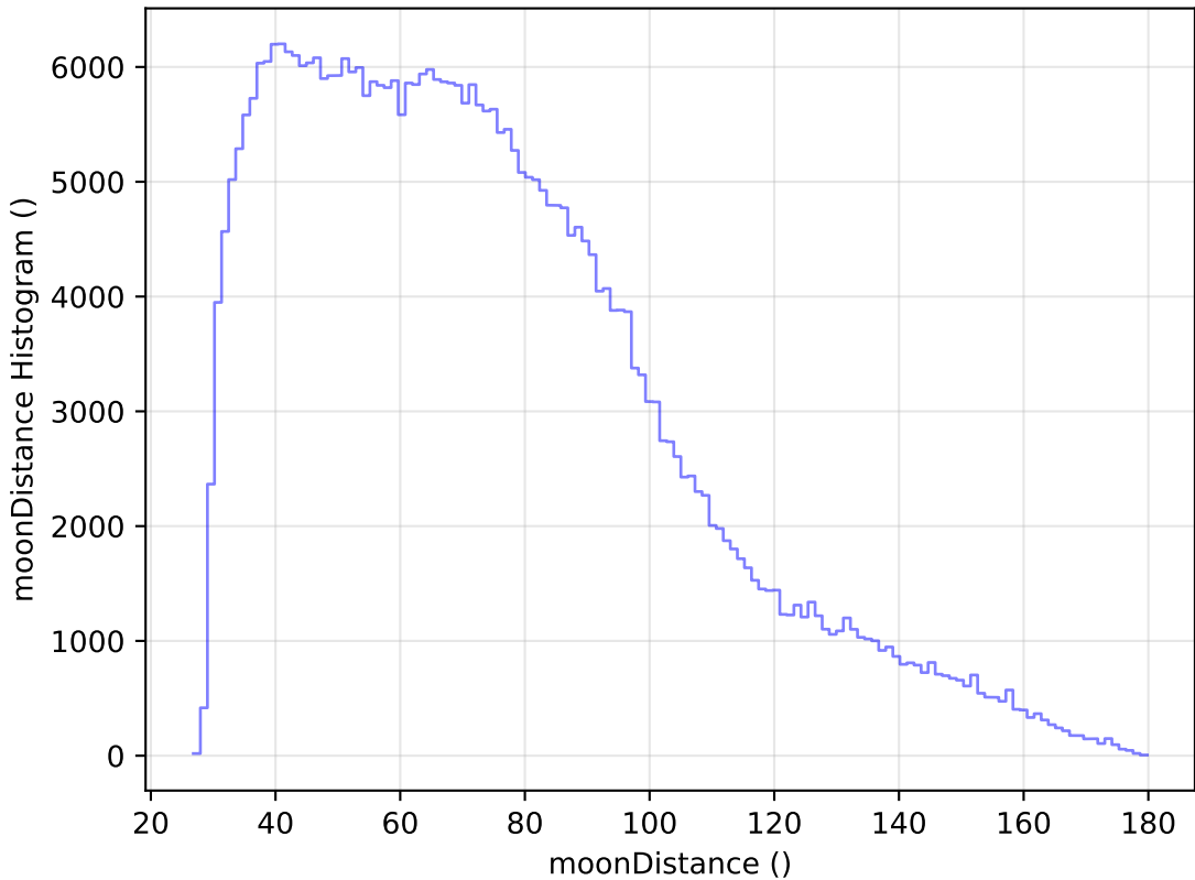
baseline_v2.1_10yrs All sky z band: moonDistance Histogram
