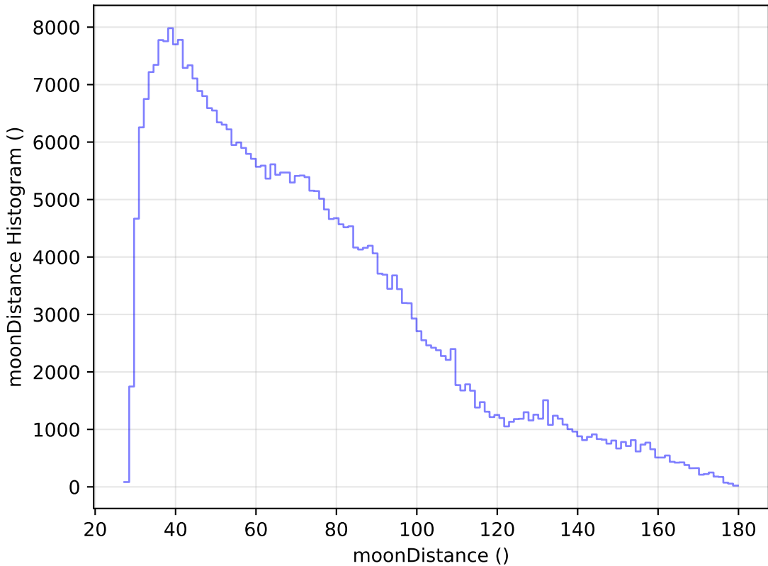
baseline_v2.1_10yrs All sky y band: moonDistance Histogram
