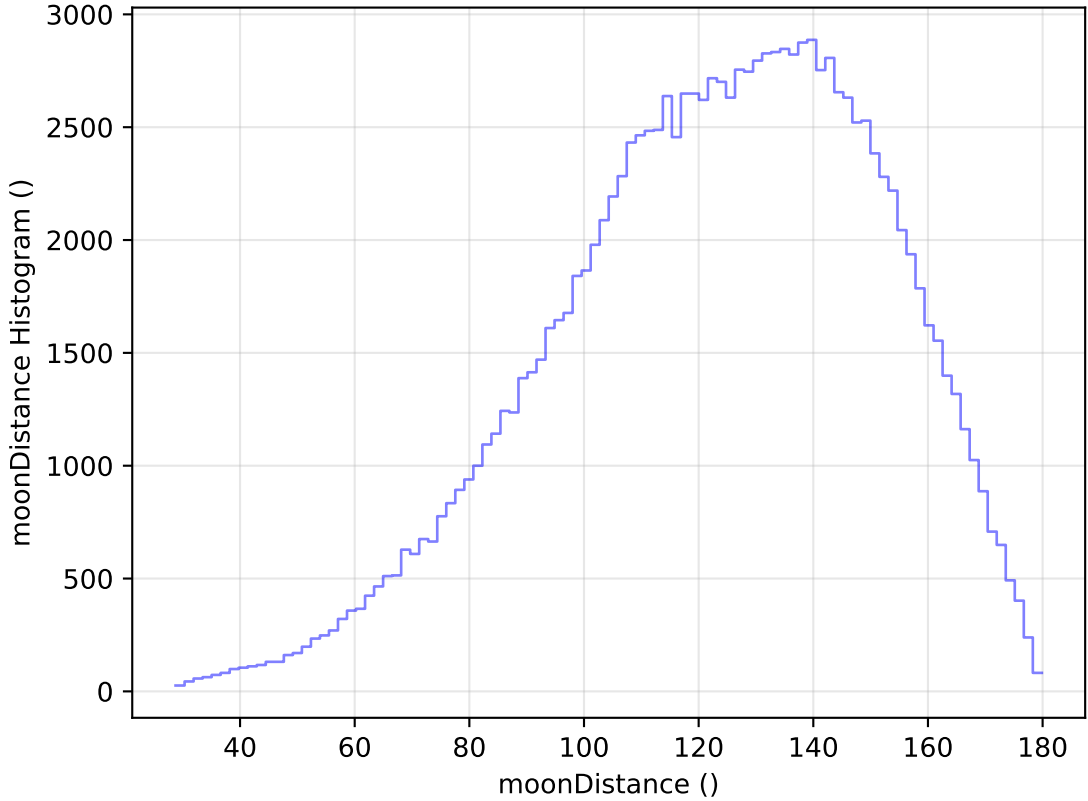
baseline_v2.1_10yrs All sky u band: moonDistance Histogram
