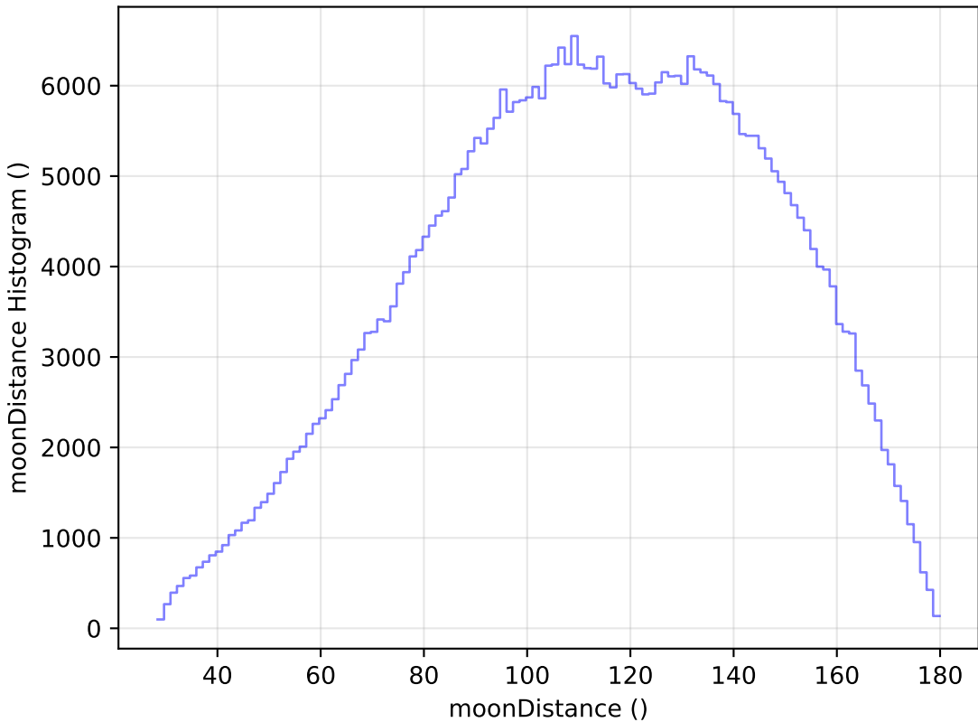
baseline_v2.1_10yrs All sky r band: moonDistance Histogram
