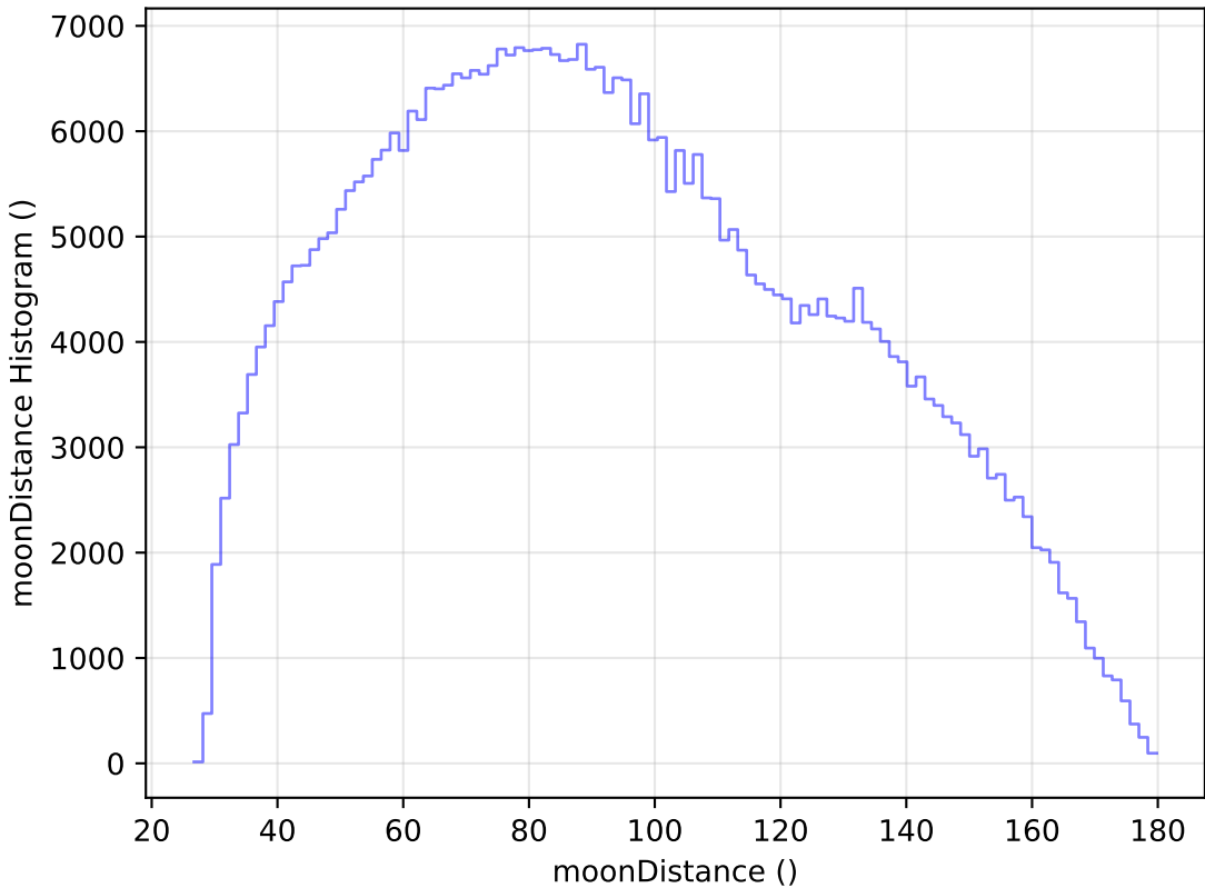
baseline_v2.1_10yrs All sky i band: moonDistance Histogram
