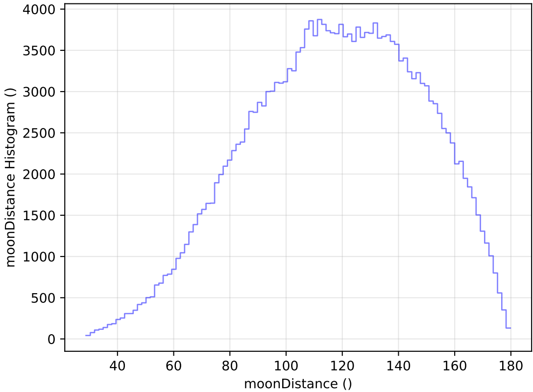
baseline_v2.1_10yrs All sky g band: moonDistance Histogram
