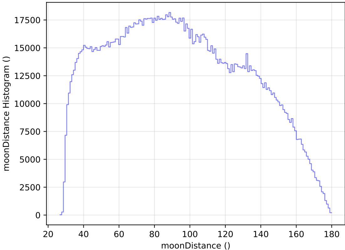
baseline_v2.1_10yrs All sky all bands: moonDistance Histogram
