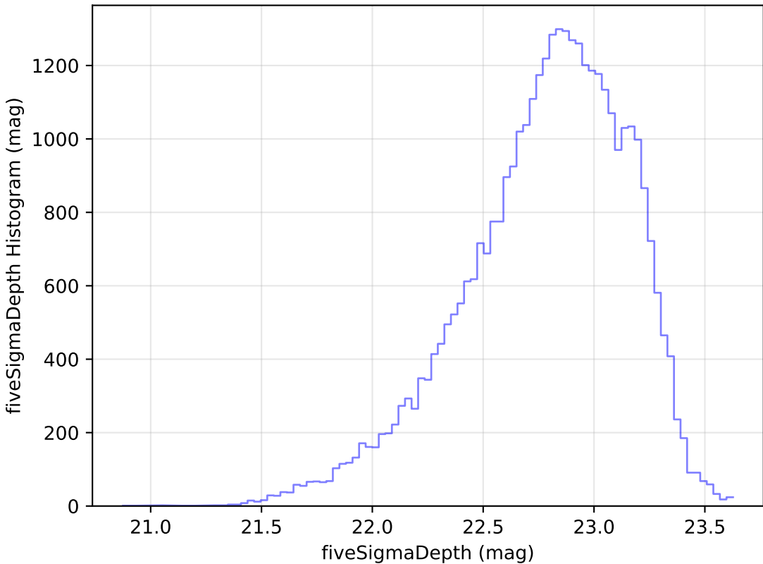
baseline_v2.1_10yrs Yr 1 z band: fiveSigmaDepth Histogram
