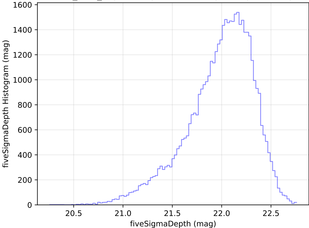
baseline_v2.1_10yrs Yr 1 y band: fiveSigmaDepth Histogram
