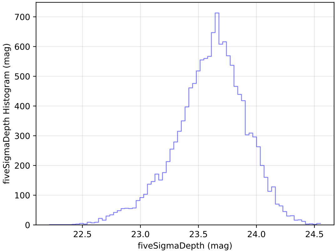
baseline_v2.1_10yrs Yr 1 u band: fiveSigmaDepth Histogram
