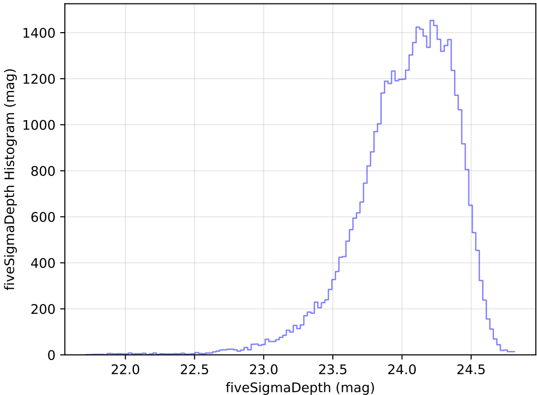
baseline_v2.1_10yrs Yr 1 r band: fiveSigmaDepth Histogram
