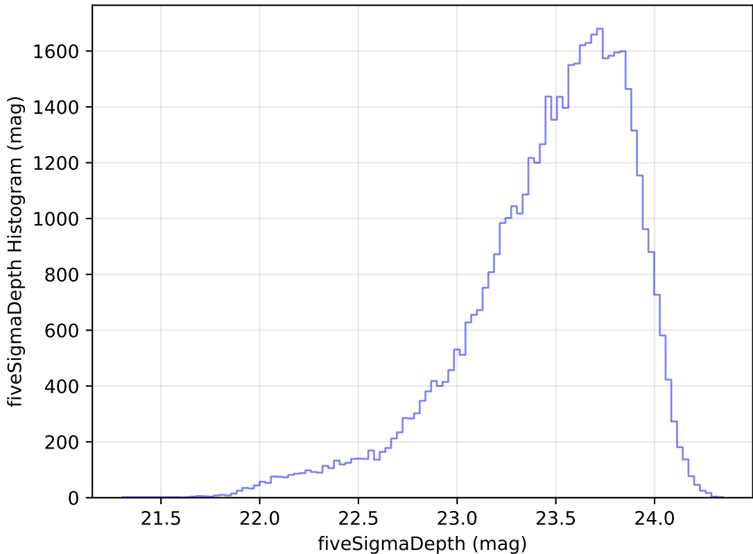
baseline_v2.1_10yrs Yr 1 i band: fiveSigmaDepth Histogram
