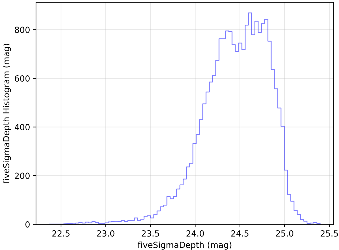
baseline_v2.1_10yrs Yr 1 g band: fiveSigmaDepth Histogram
