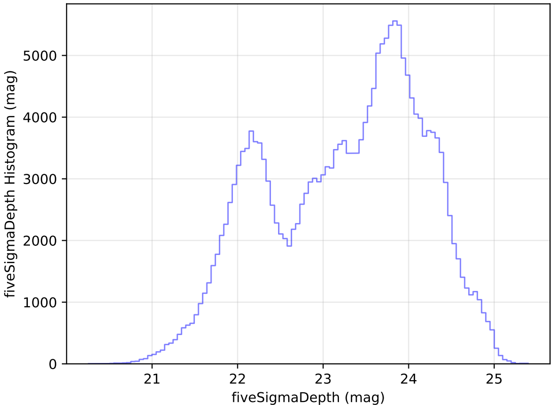
baseline_v2.1_10yrs Yr 1 all bands: fiveSigmaDepth Histogram
