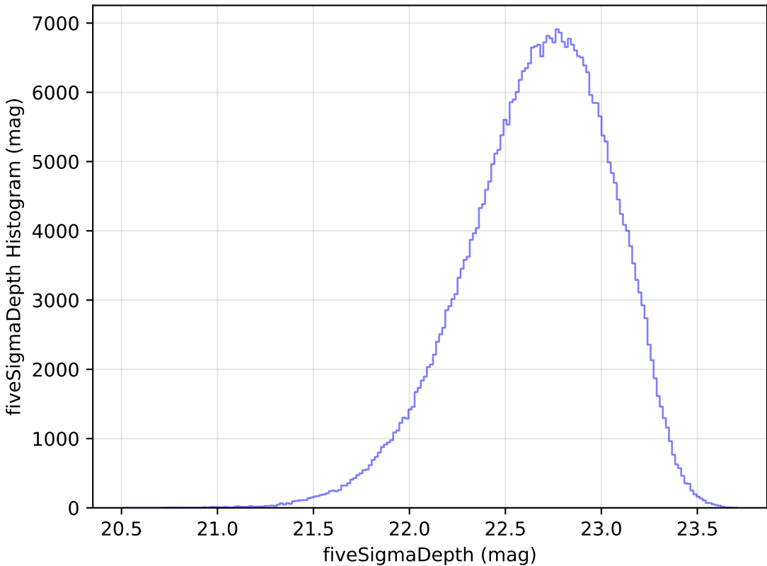
baseline_v2.1_10yrs WFD z band: fiveSigmaDepth Histogram
