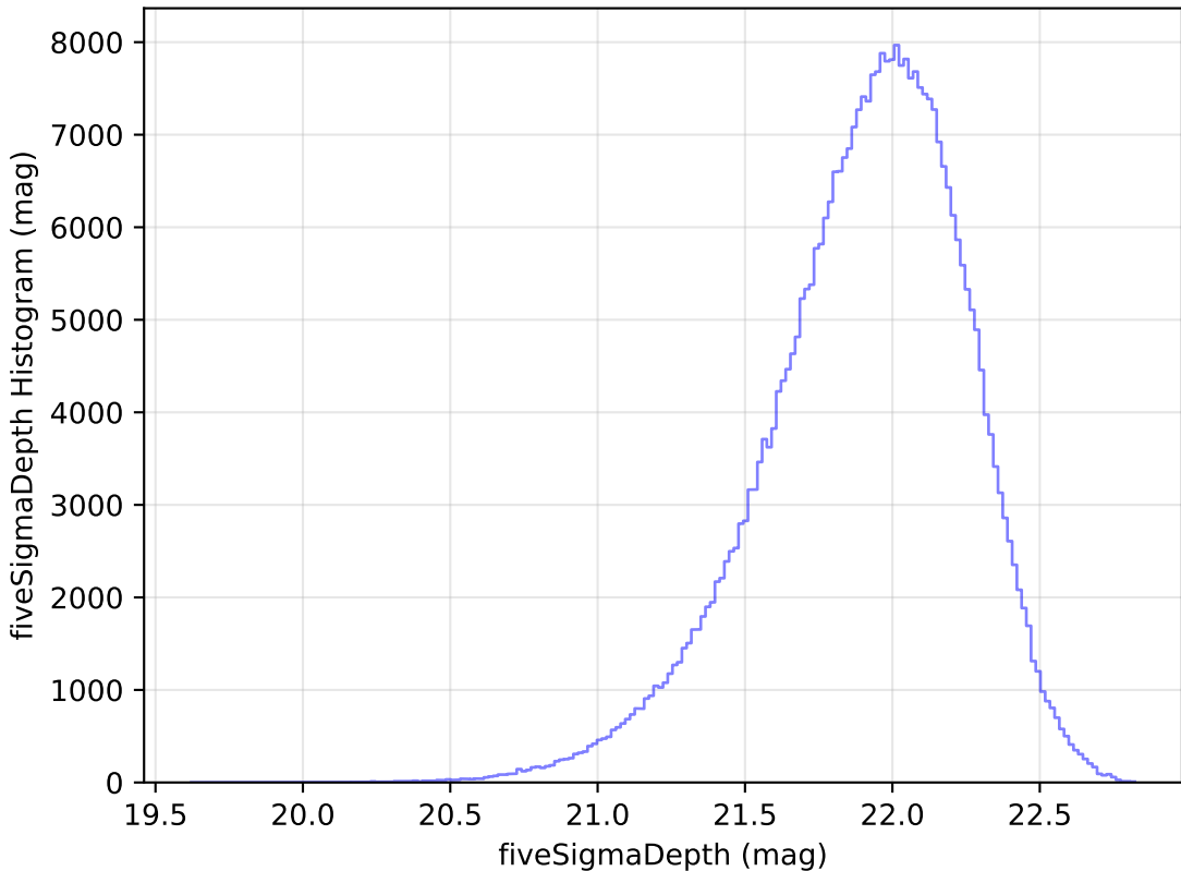
baseline_v2.1_10yrs WFD y band: fiveSigmaDepth Histogram
