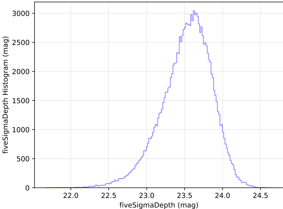
baseline_v2.1_10yrs WFD u band: fiveSigmaDepth Histogram
