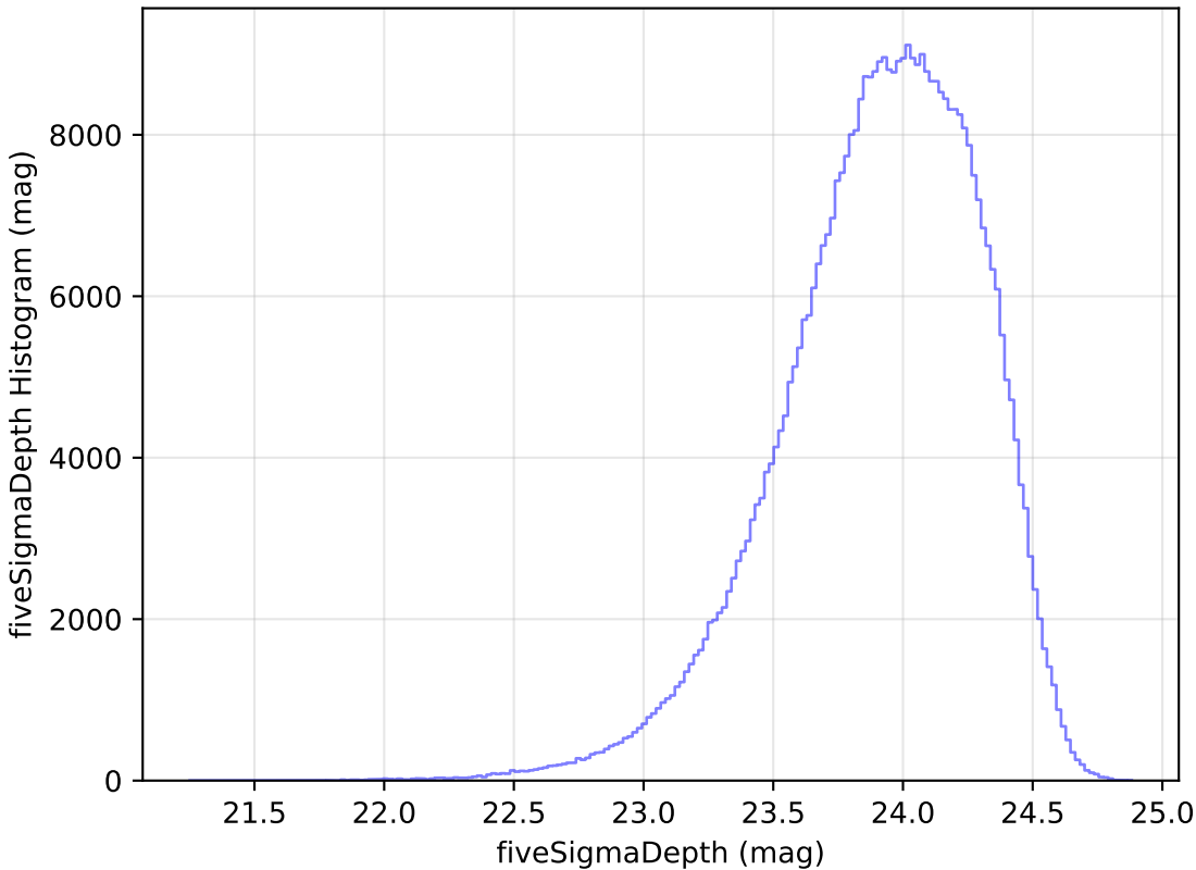
baseline_v2.1_10yrs WFD r band: fiveSigmaDepth Histogram
