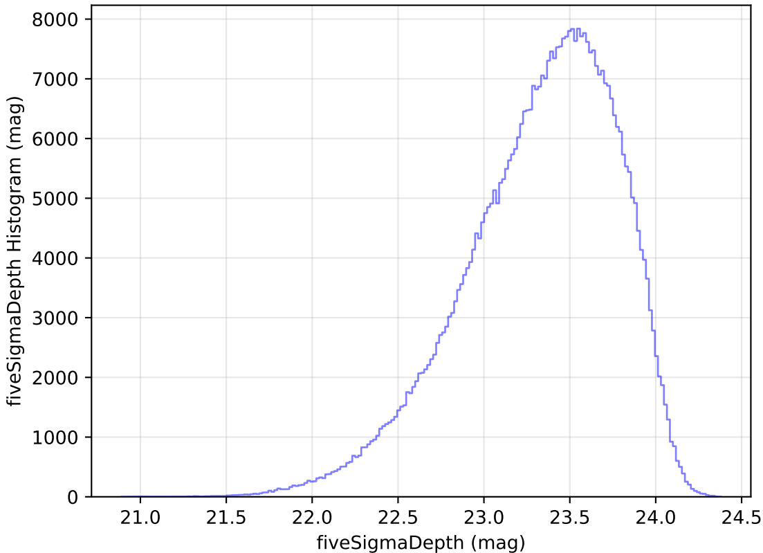
baseline_v2.1_10yrs WFD i band: fiveSigmaDepth Histogram
