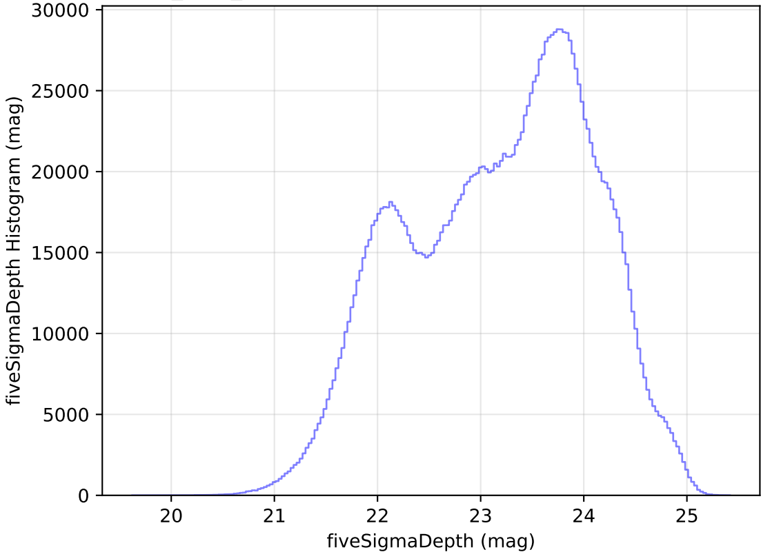
baseline_v2.1_10yrs WFD all bands: fiveSigmaDepth Histogram
