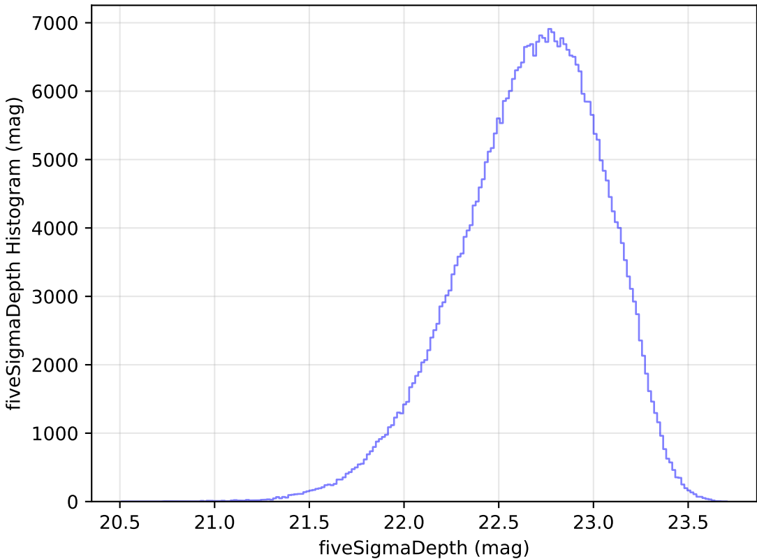
baseline_v2.1_10yrs All sky z band: fiveSigmaDepth Histogram
