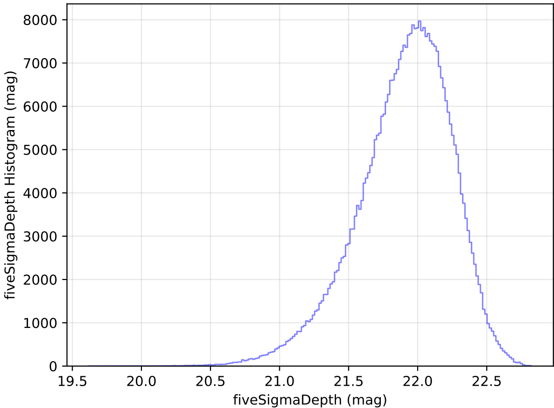
baseline_v2.1_10yrs All sky y band: fiveSigmaDepth Histogram
