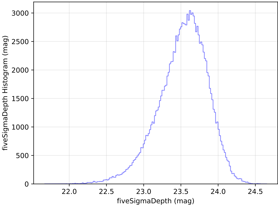
baseline_v2.1_10yrs All sky u band: fiveSigmaDepth Histogram
