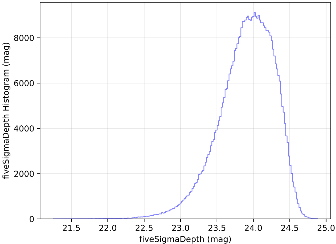
baseline_v2.1_10yrs All sky r band: fiveSigmaDepth Histogram
