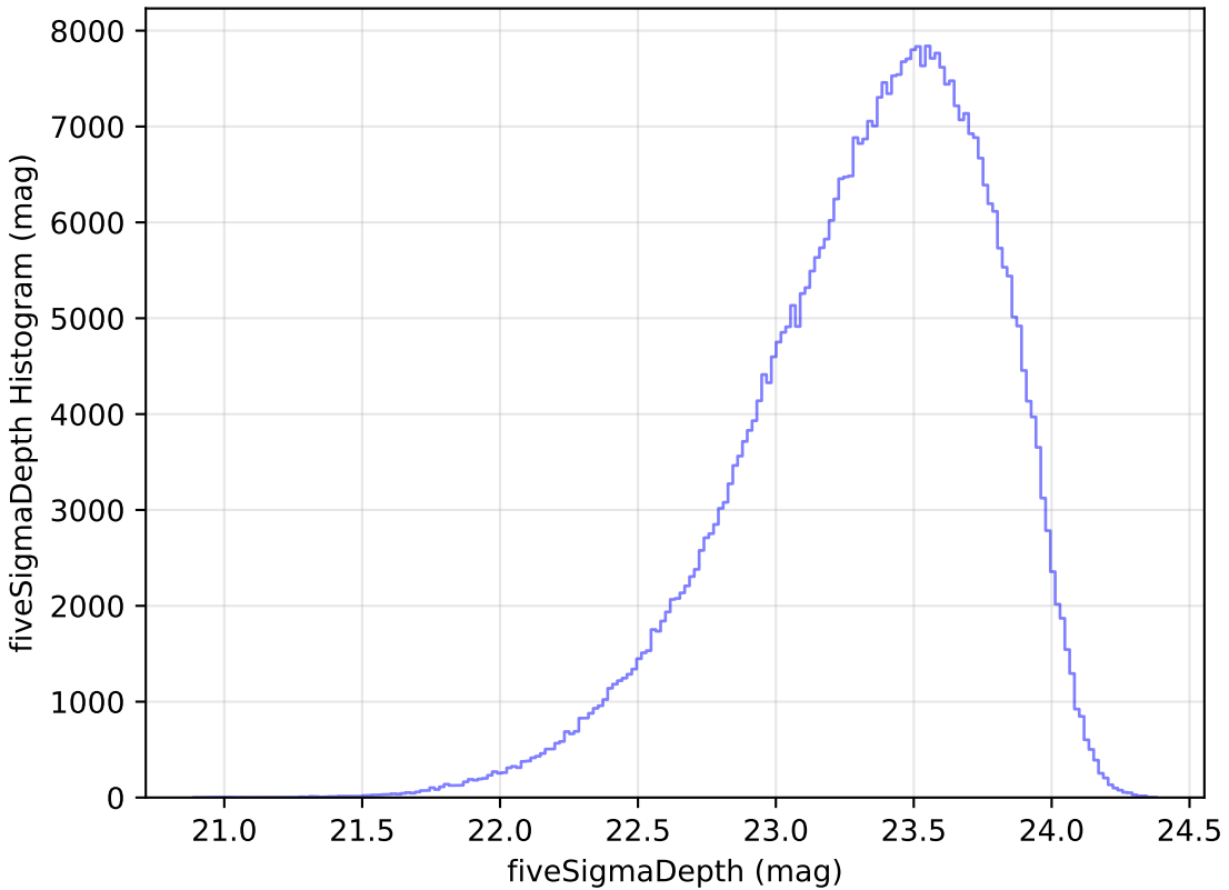
baseline_v2.1_10yrs All sky i band: fiveSigmaDepth Histogram
