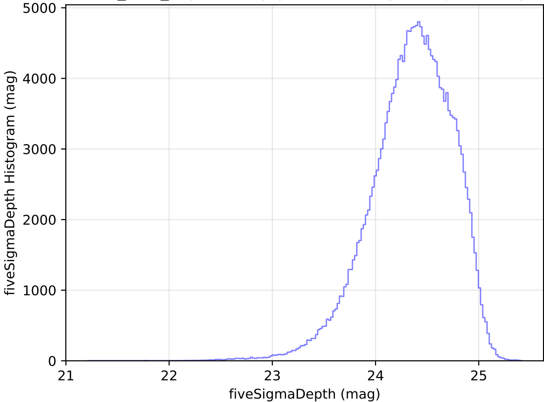
baseline_v2.1_10yrs All sky g band: fiveSigmaDepth Histogram
