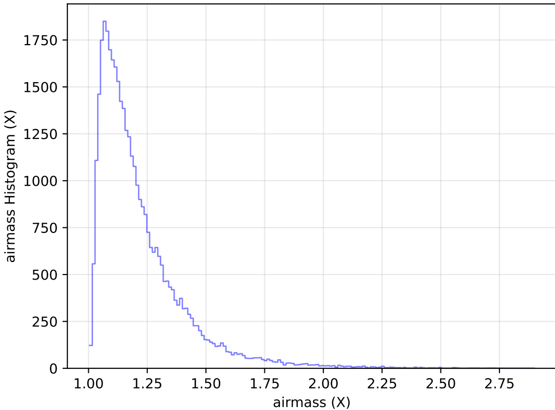
baseline_v2.1_10yrs Yr 1 z band: airmass Histogram
