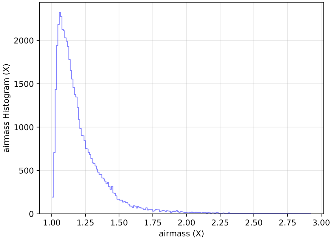
baseline_v2.1_10yrs Yr 1 i band: airmass Histogram
