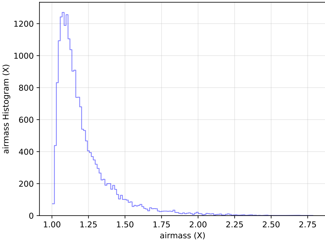
baseline_v2.1_10yrs Yr 1 g band: airmass Histogram
