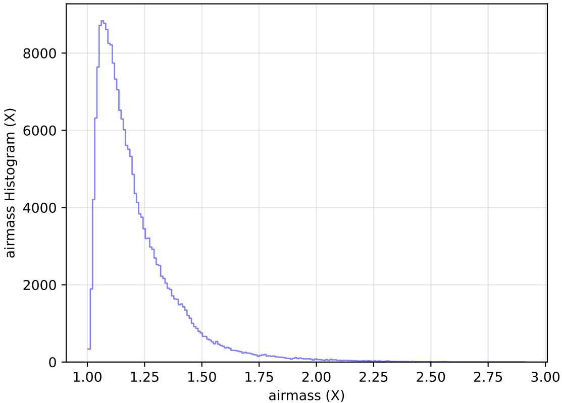
baseline_v2.1_10yrs Yr 1 all bands: airmass Histogram
