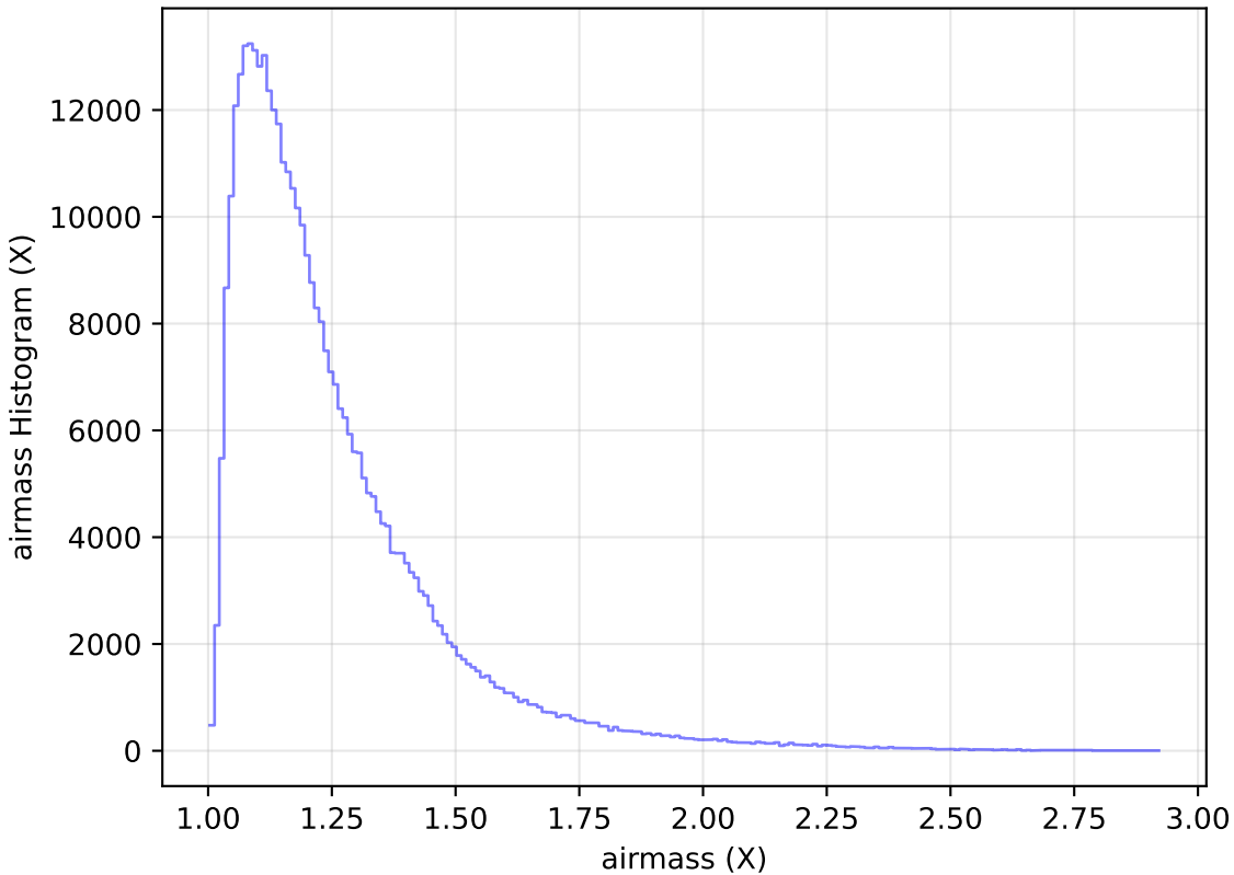
baseline_v2.1_10yrs WFD z band: airmass Histogram
