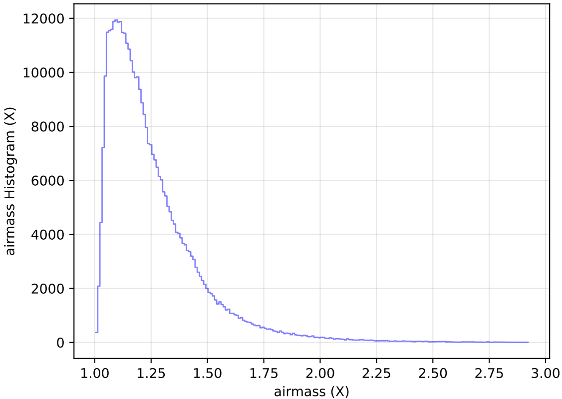
baseline_v2.1_10yrs WFD y band: airmass Histogram
