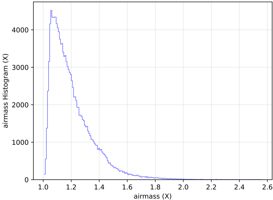
baseline_v2.1_10yrs WFD u band: airmass Histogram
