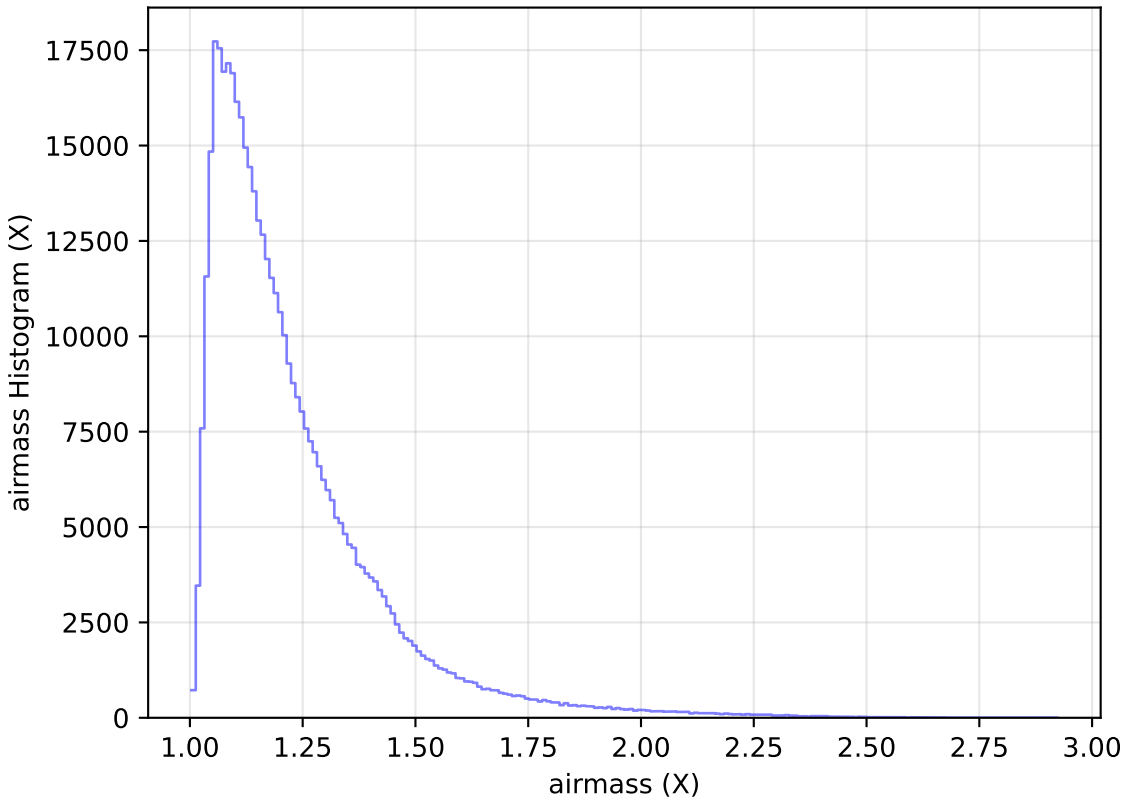
baseline_v2.1_10yrs WFD r band: airmass Histogram
