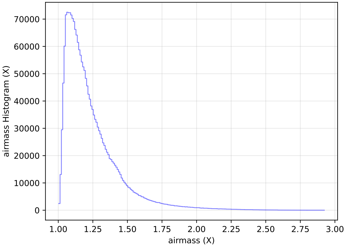
baseline_v2.1_10yrs WFD all bands: airmass Histogram
