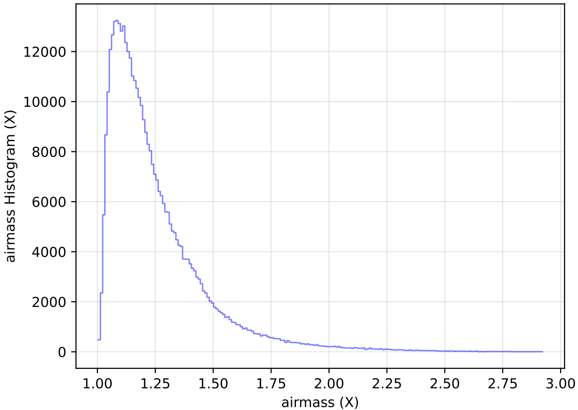
baseline_v2.1_10yrs All sky z band: airmass Histogram
