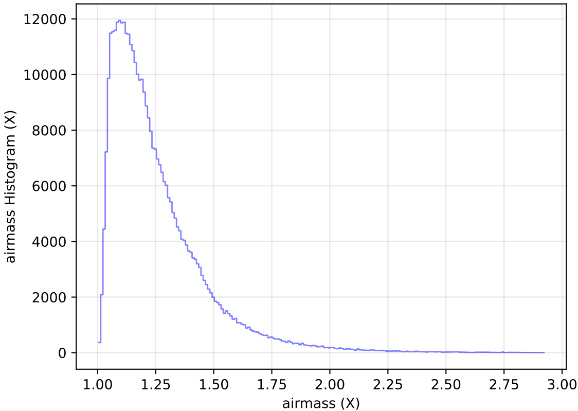
baseline_v2.1_10yrs All sky y band: airmass Histogram
