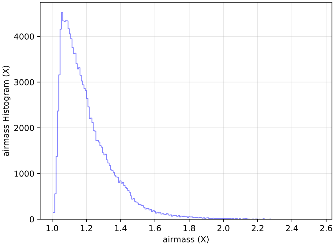
baseline_v2.1_10yrs All sky u band: airmass Histogram
