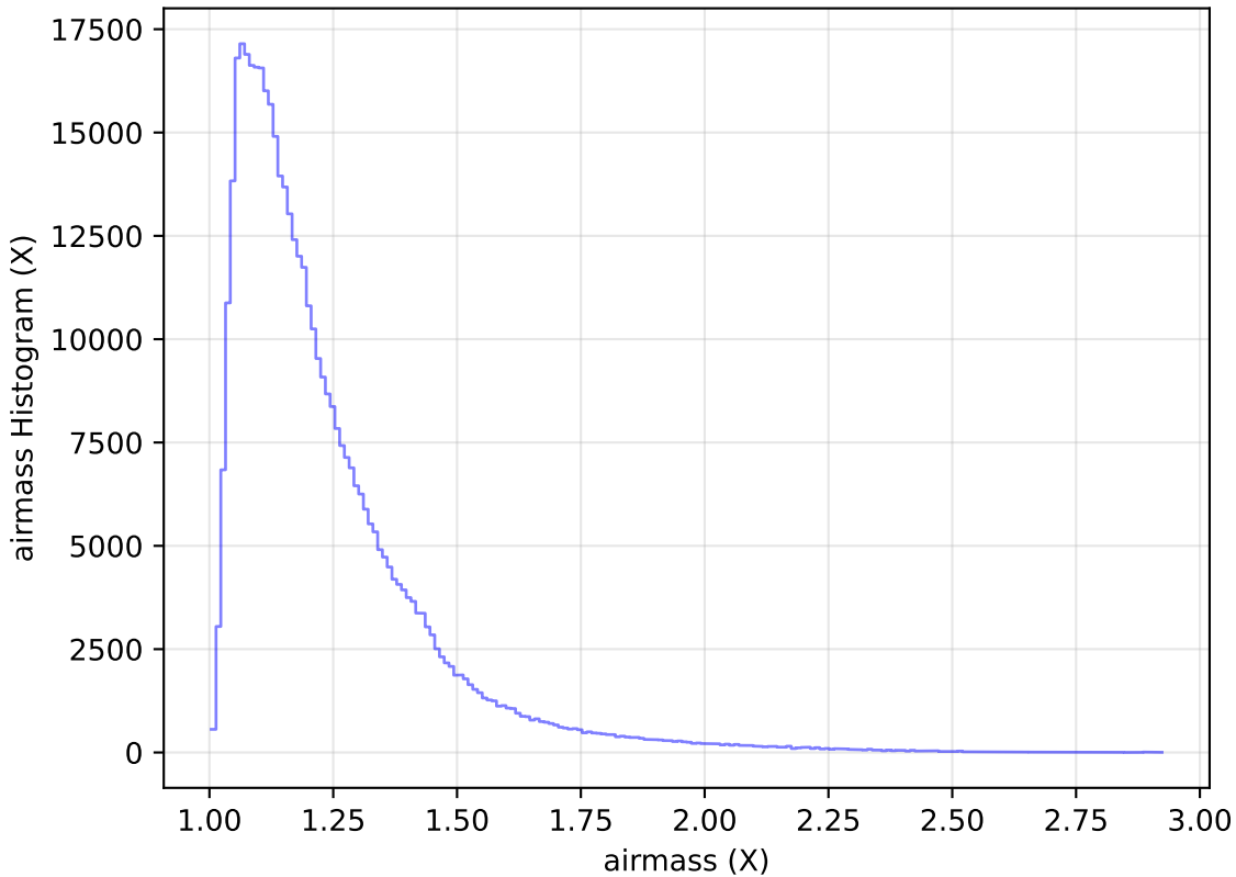
baseline_v2.1_10yrs All sky i band: airmass Histogram
